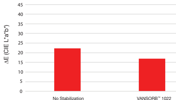
Scented soy wax candle formulation containing 0.2 wt% of VANSORB™ 1022 in a light box with continuing exposure to black light for 72 hours.
